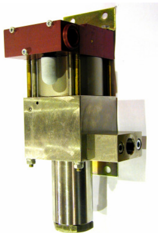
MSF12(L) single acting, single air drive head and distance piece (Standard= Bottom inlet)
