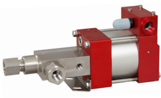
MSF72(L) single acting, single air drive head and distance piece (Standard= Bottom inlet)
