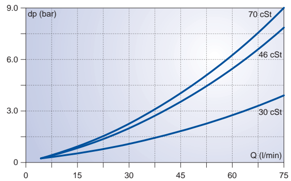
Q = 7.5 ... 75 l/min
