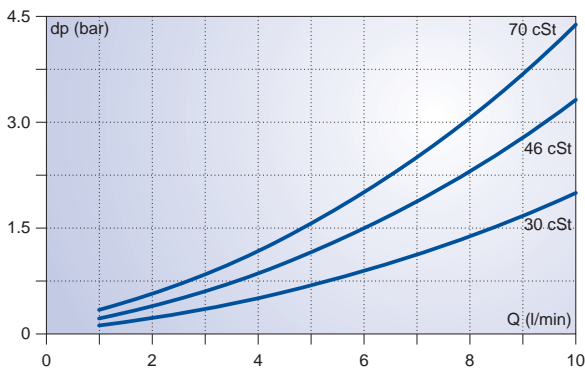
Q = 1.0 ... 10 l/min
