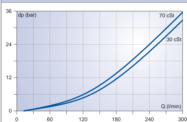
Q = 15 ... 300 l/min
