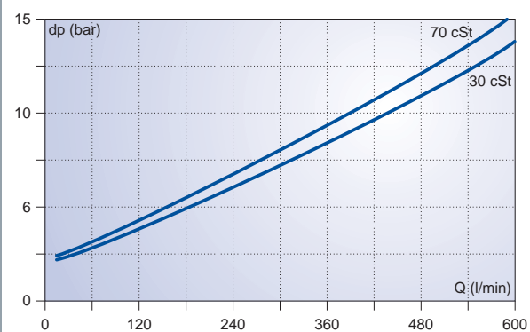
Q = 12 ... 600 l/min
